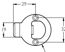
PT482/SP Drive-in Strike Plate
