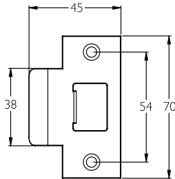
PT480/SPT Universal Strike Plate
